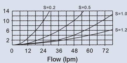
Pressure Drop (bar) R-E
